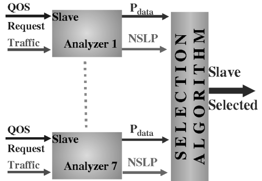
Fig. 2. Polling scheme at the master side
