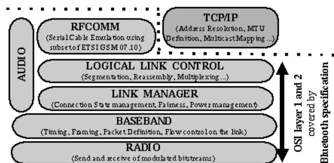
Fig. 1. Bluetooth Stack
