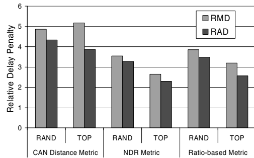
Fig. 4. Relative delay penalty for CAN tree-based multicast with and without topology-aware optimizations using a d=8, z=10 CAN configuration.
